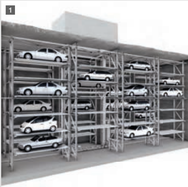
1 MasterVario R3C with sideways storage
